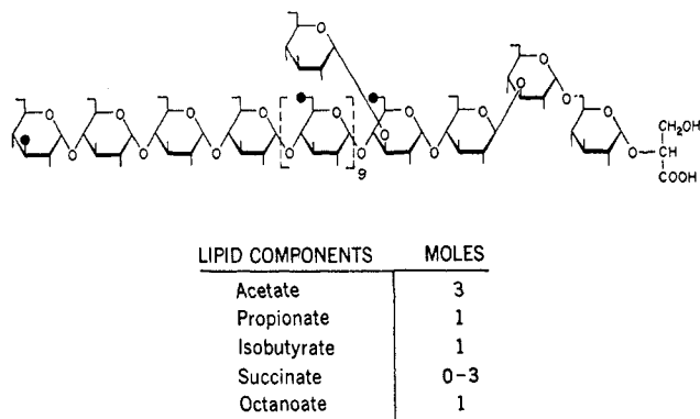
Figure 3. Structure of the polysaccharide component from the methylglucose lipopolysaccharide from Mycobacterium phlei and a list of the acyl groups which form the lipid component. The closed circles stand for O -methyl groups. All sugars have the D -glucose configuration. Although the exact distribution of the acyl groups is unknown, they appear to be esterified mainly to the primary hydroxyl groups of the glucose residues.
