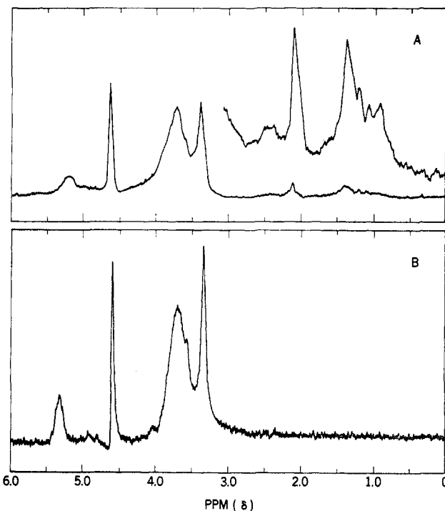
Figure 5. Nuclear magnetic resonance spectra (Varian A-60) of the lipopolysaccharide (A) and the polysaccharide (B) in deuterium oxide. The line at 4.6 ppm is HDO, the anomeric protons of the sugars are at 5.4 ppm, the ring protons of the sugars at about 3.7 ppm, the O -methyl groups at 3.3 ppm, and the acyl groups in the region 1-2.5 ppm.
